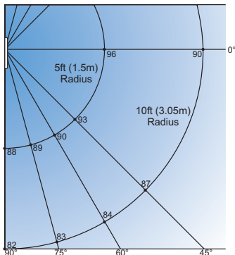
Genesis Series Cone Speaker/strobe
